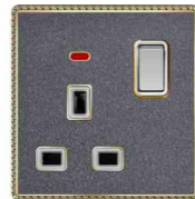
K8-042 13A switched socket w/without neon
